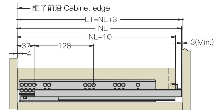
外置抽屉 Standard drawer
